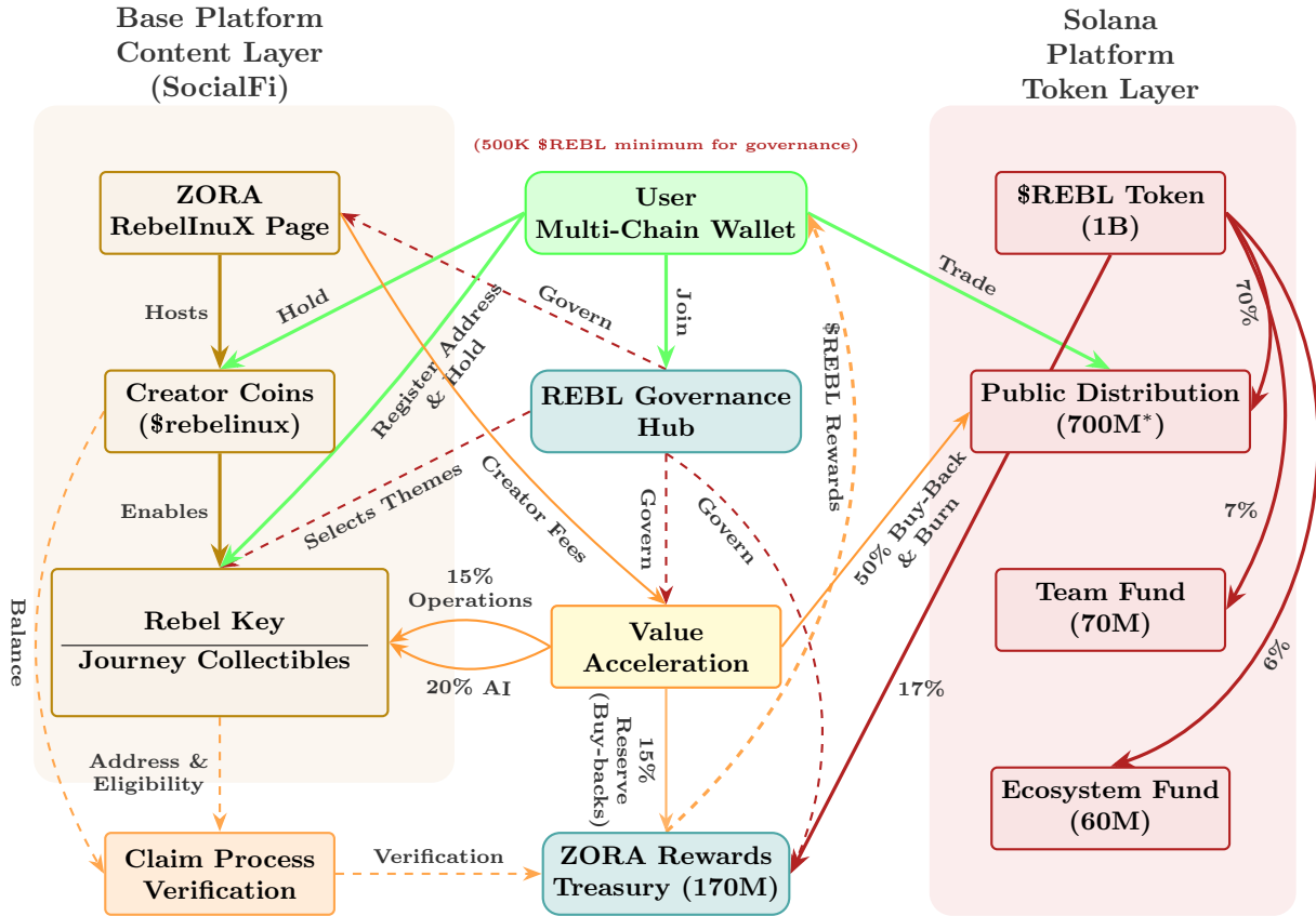
Figure 1: RebelInuX multi-chain architecture showing the Base content layer (Creator Coin + Digital Collectible Bundle), Solana token layer, and core value flows. All Value Acceleration deployments are triggered by REBL Governance Hub vote.
